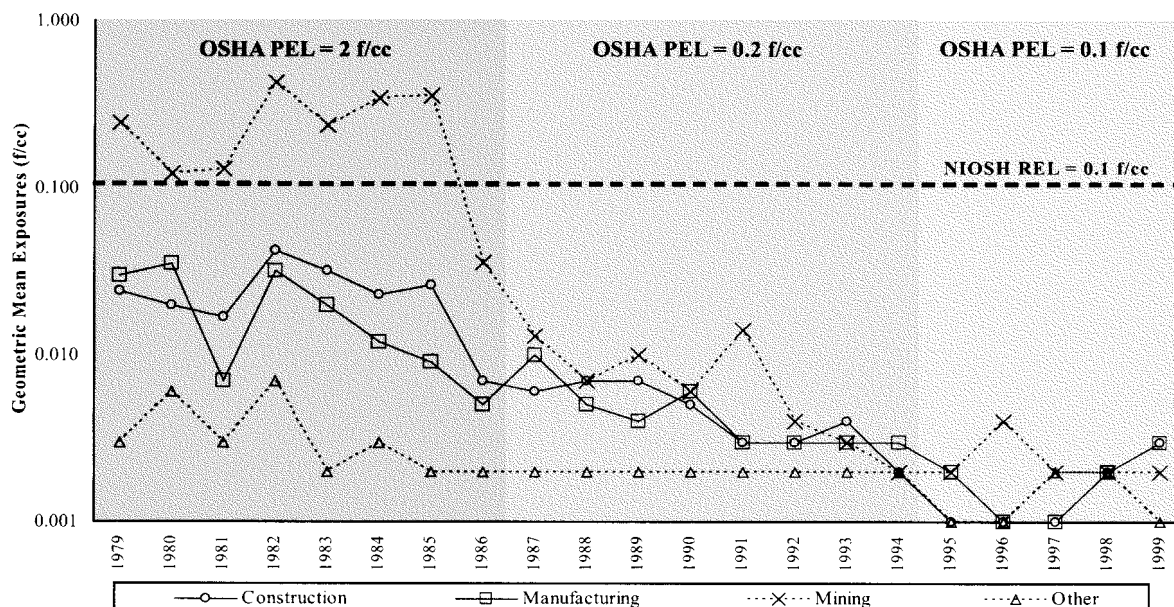
Chart VIII-1: Industry Trends of Airborne Asbestos Concentrations. 89
