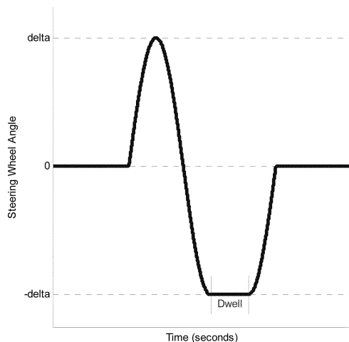
Figure 3: Sine with Dwell profile
