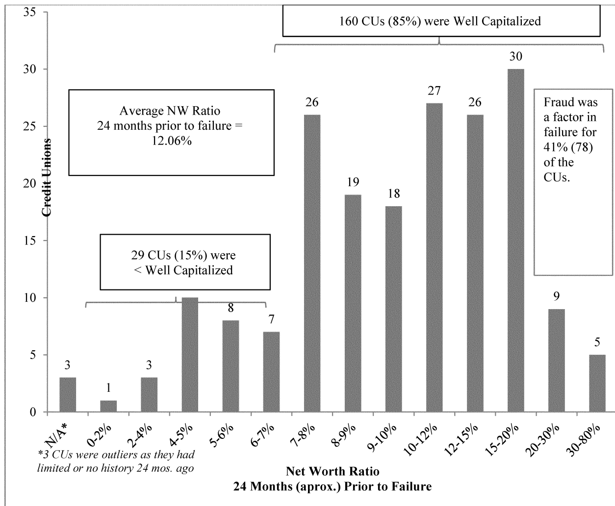
Net Worth Ratio 24 Months Prior to Failure (All CU Failures in the Last 10 Years)
